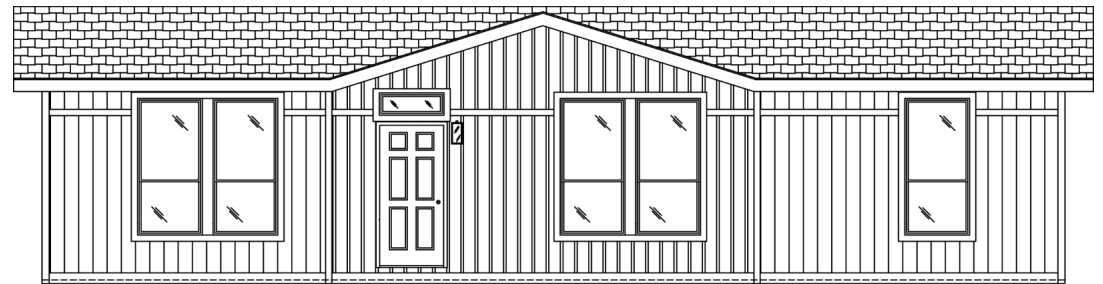
FRONT SIDEWALL
