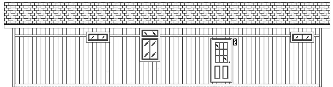
BACK SIDEWALL
